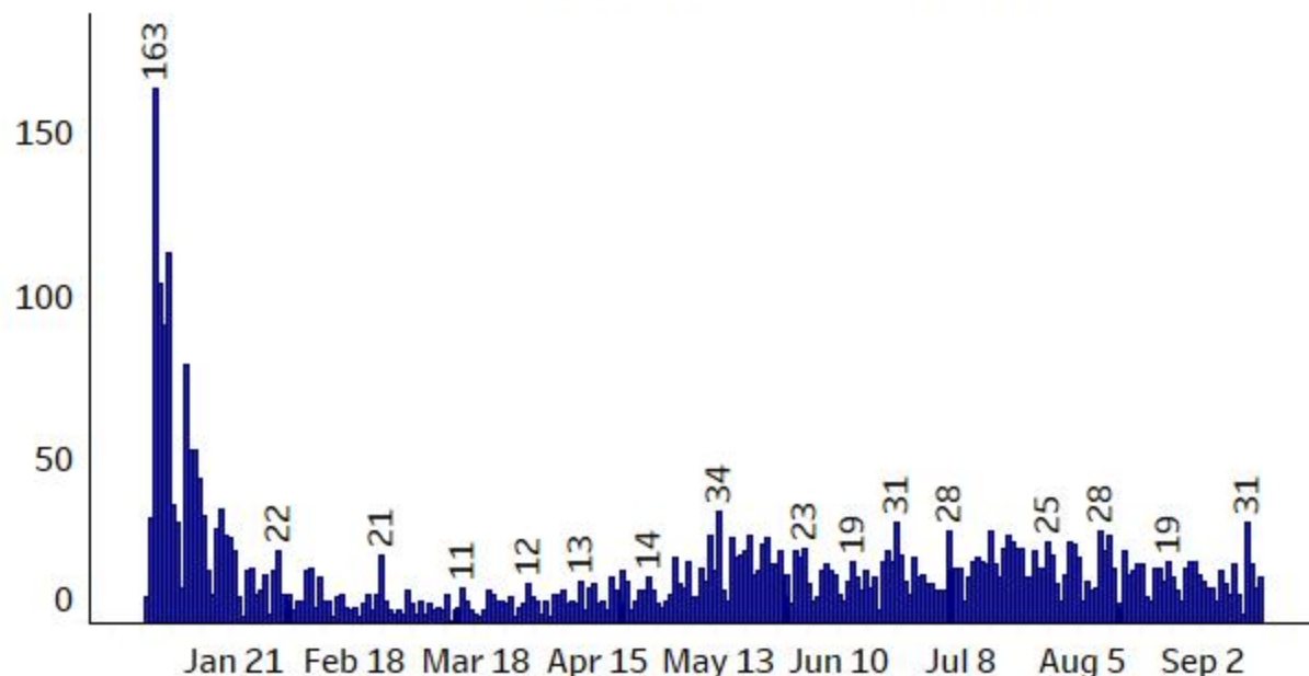
Case Trends (01/01/2021 - 09/20/22)
