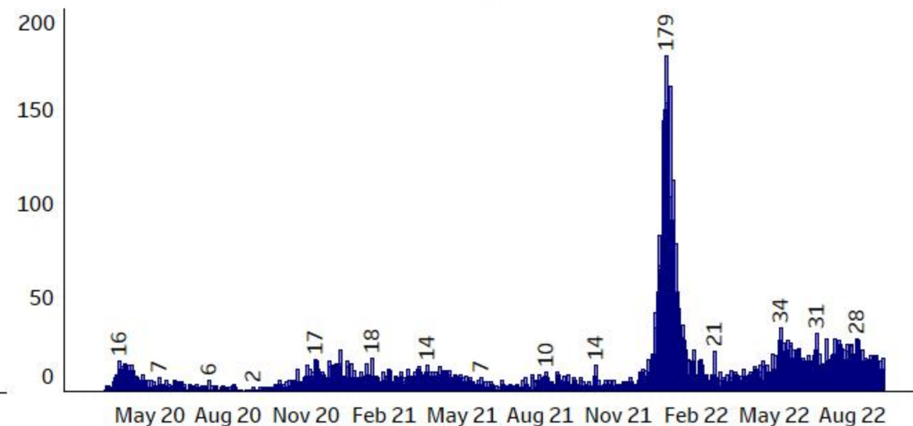
Case Trends (1/1/2020 - 09/20/22)
